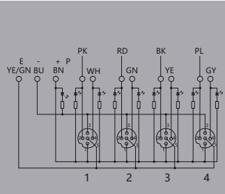
M12-A3-4K5N-3.0PVC/GY Circuit
