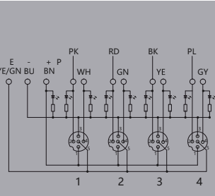
M12-A3-4K5P-3.0PVC/GY Circuit
